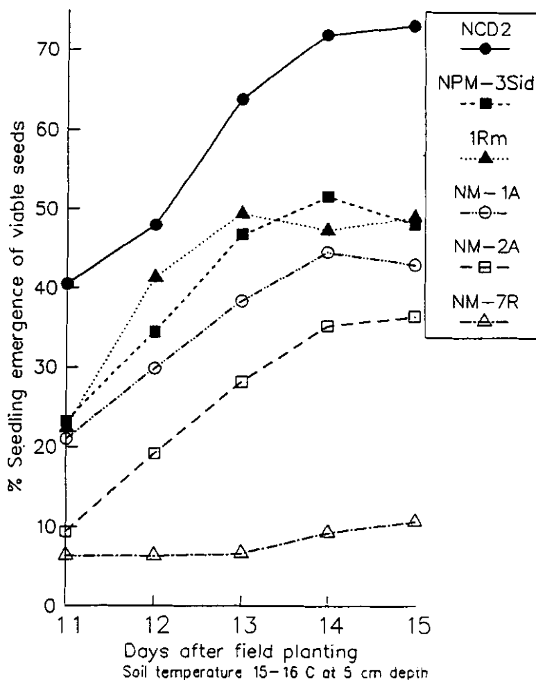
Figure 1. Pearl millet seedling field emergence of cold tolerant and susceptible varieties in 1998.
