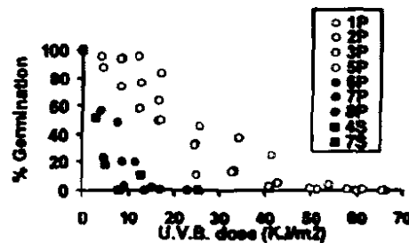
Figure 3. Effect of UVB dose on survival of conidia of C. africana . (Open circles indicate germination was in light; solid shapes, dark; P, primary conidia; S, secondary conidia).
