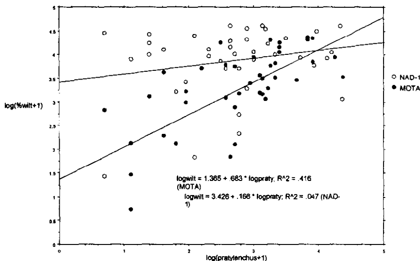
Figure 1. Relationship between Pratylenchus zea and acremonium wilt on sorghum in Niger, 1997 cropping season.
