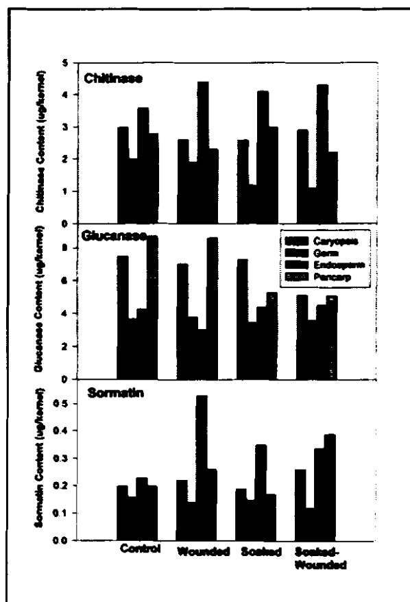
Figure 4. Effects of treatments on chitinase, glucanase and sormatin levels in sorghum caryopsis and tissues (average over cultivar and age).
